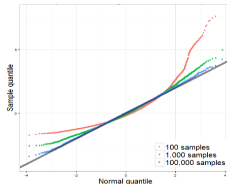
Figure 4: QQ-norm plot for averages of different sample sizes showing convergence to Normal when skewness is 18.2 for Revenue/user. Actual data used
